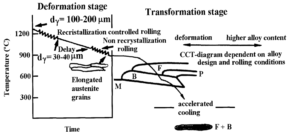
Fig. 6 Schematic representation of the thermomechanical controlled rolling and accelerated cooling procedure applied to API 5L X-70 slabs
